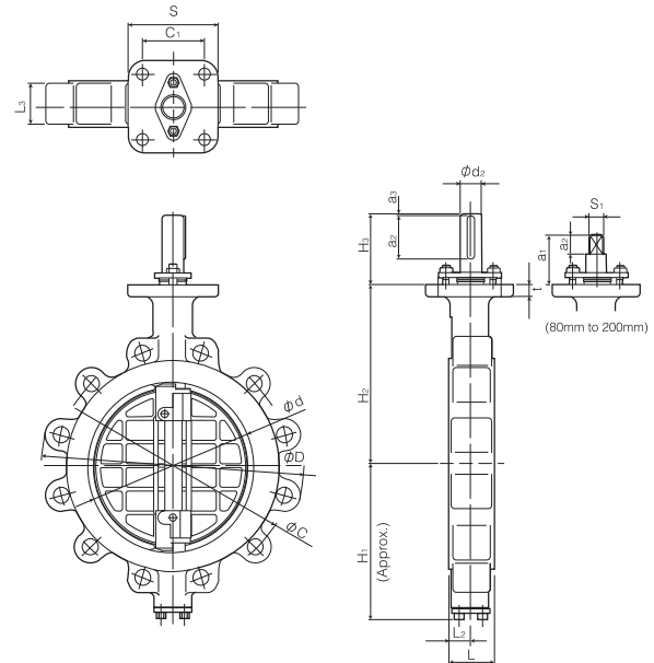
Lugged type 304Q
