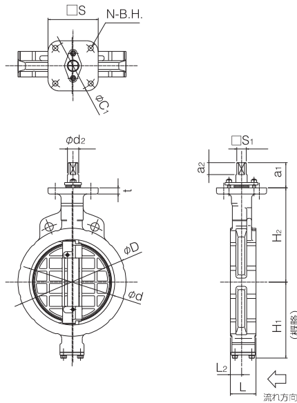
Wafer type 304A
